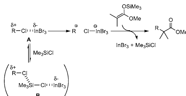
Scheme 2. Plausible Mechanism
