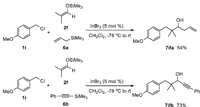
Scheme 3. Three-Component Tandem Reaction
